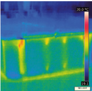
Heat leak test performed with the Nordic Insulation System
